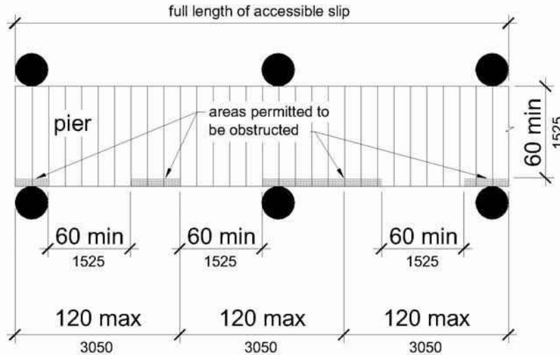
Fig. 59 Pier Clearances
