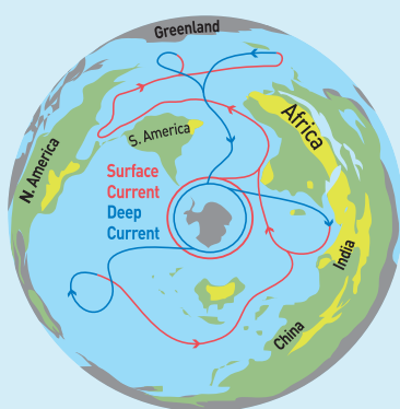
Figure 2. Example of a global conveyor belt.
