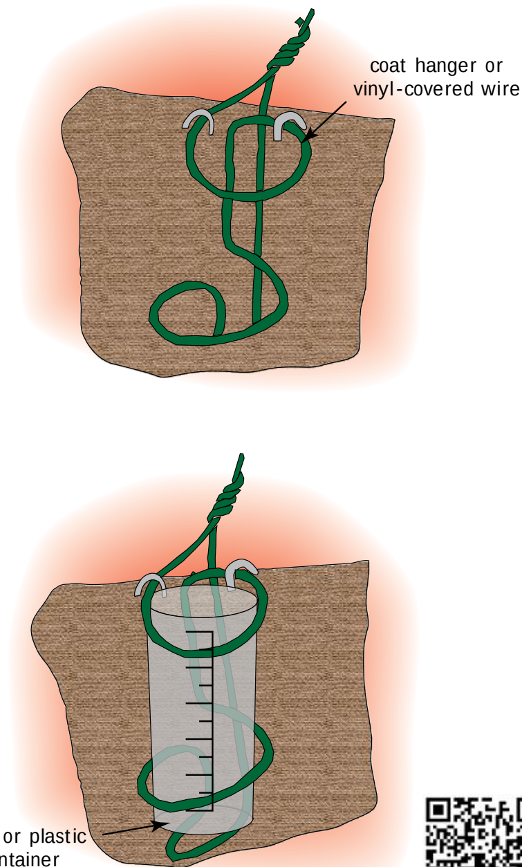
Figure 4. Rain Gauge
